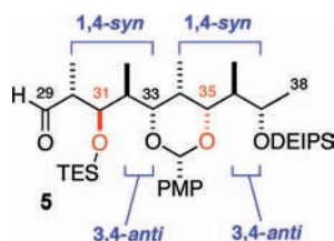
Figure 1. Stereotetrads embedded in the C29–C38 segment.
